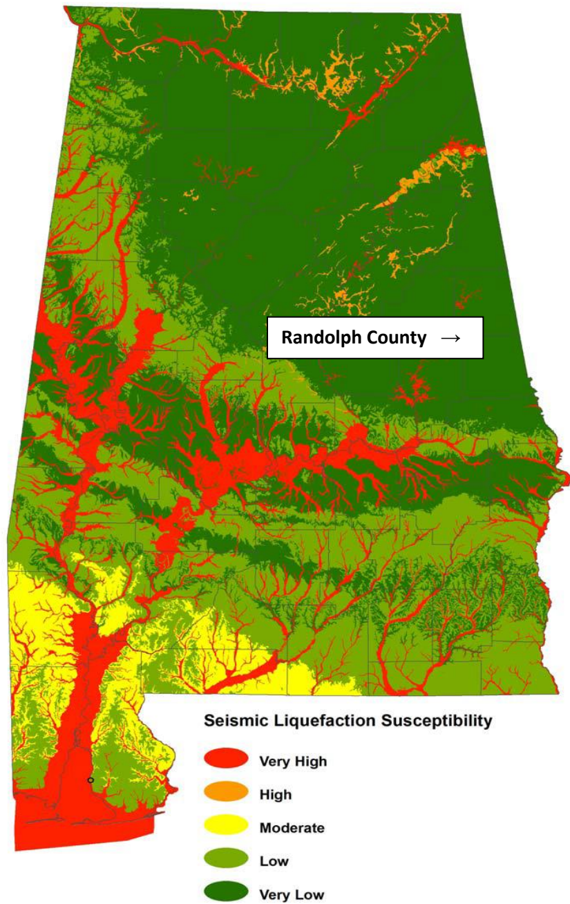
Figure 4-9: Seismic Liquefaction Susceptibility
